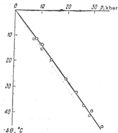
FIG. 3. Shift of the Curie temperature of gadolinium with pressure.
